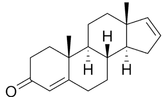
Structure of androstadienone
